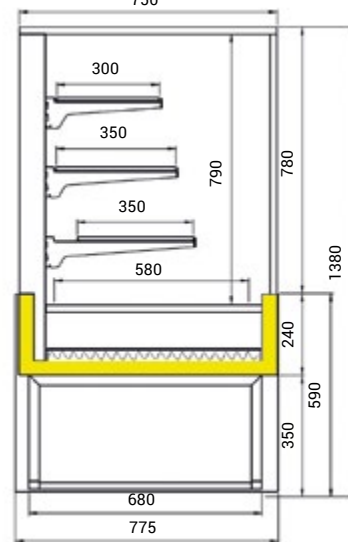
bokorys Kristall HOT
