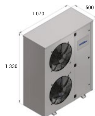
▼ FSC 1065, FSC 1165
