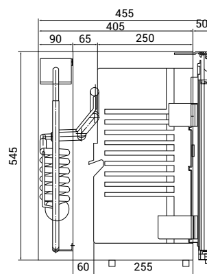
bokorys TM 42
