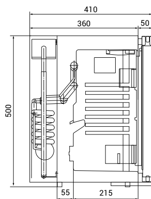
bokorys TM 32
