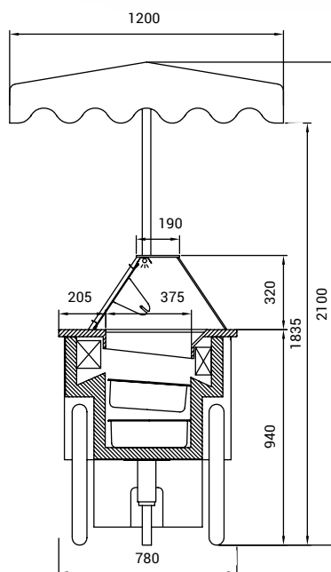
bokorys Riksha K-1 RK7
