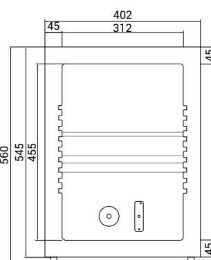
bokorys TM 42
