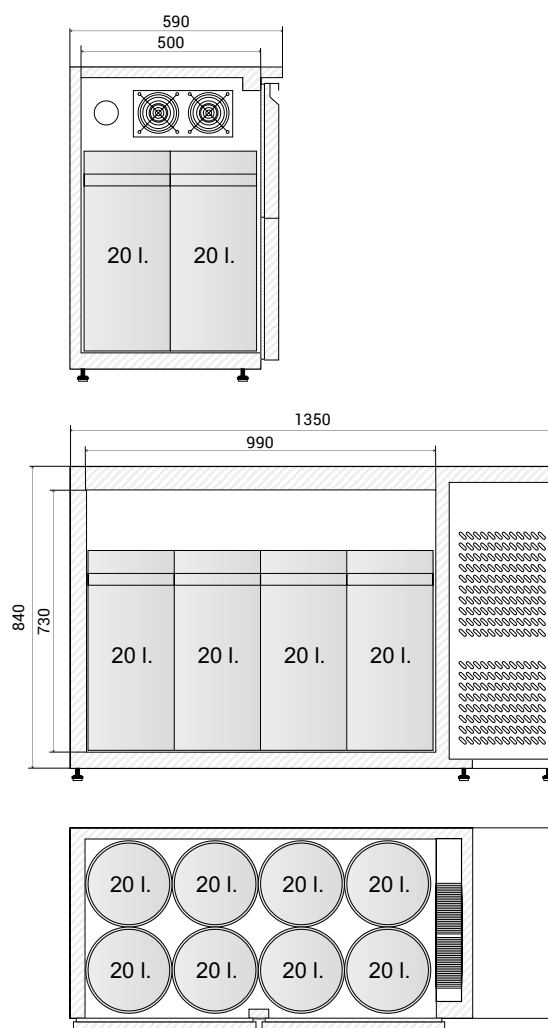
bokorys CKC8 KEG
