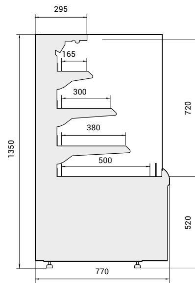
Carina 06 SELF bokorys
