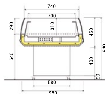
bokorys Artemis
